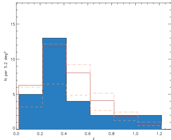
Figure 13. Impact of the steepening of the M - T relation in the group regime on the modelling of the cluster number density. The full line corresponds to our fiducial model (broken power law, Section 5.1), giving 6.2 clusters per square degree. If we assume the Vikhlinin et al (2006) result (single slope of 1.5, dashed line), the cluster density drops to 3.6 deg -2 . The relation of Arnaud et al. (2005), motivated by a possible steepening of the mass function below 3.5 keV (single slope of 1.7, dash-dotted line), seems to be closer to our observations and yields a cluster density of 6.9 deg -2 .
