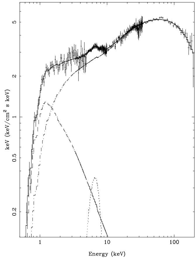
FIG. 3.—Broadband EF_E spectrum during the HS (crosses). Histograms show the model components caused by two thermal-Compton plasmas with Compton reflection and a broad Gaussian (see § 4.2 and Table 4).
