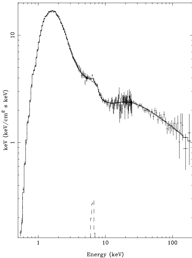
FIG. 5.—Broadband EF_E spectrum during the SS (crosses). Histograms show the continuum model with the hybrid plasma Compton upscattering blackbody disk photons and a broad disk line.
