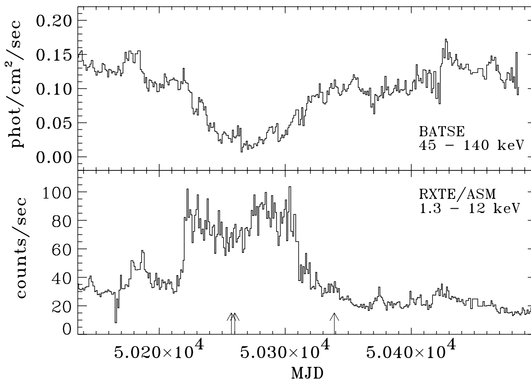
FIG. 1.—One-day-average light curve of Cyg X-1 detected with the CGRO /BATSE and RXTE /ASM during the 1996 state transitions. (From the public archives at coss.c.gsfc.nasa.gov/batse/hilev/occ.html and xte.mit.edu/XTE/asmlc/ASM.html , respectively.) BeppoSAX observations are indicated with arrows.
