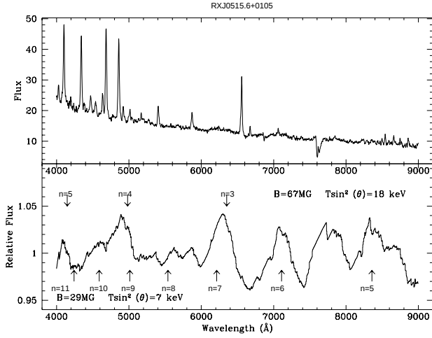
Fig. 3. Upper panel: The difference spectrum between spectra at 0.48 and 0.99 orbital phases. Ordinates are in units of 10^{-16} \text{ erg cm}^{-2} \text{ s}^{-1} \text{ Å}^{-1} . Lower panel: The smoothed normalized cyclotron spectrum and the expected positions for the two best solutions of B and T \sin^2(\theta) as described in the text.
