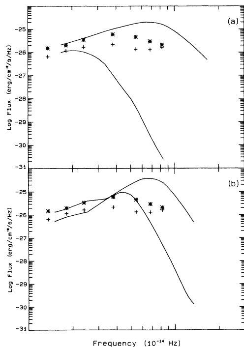
FIG. 9.—Comparison of our estimate of the cyclotron flux with literature best fits. The data shown in both panel for phase 0.0 ( crosses ) and phase 0.5 ( stars ) have been derived from our light curves in the B , V , I , J , H , and K bands, and from a single U measurement (see text for details). Solid curves represent the best fit at the two phases, as derived from the models of (a) Wickramasinghe & Meggitt 1985, and (b) Cropper et al. 1986. Curves have been arbitrarily scaled to match our measurements in the IR range ( H and K bands).
