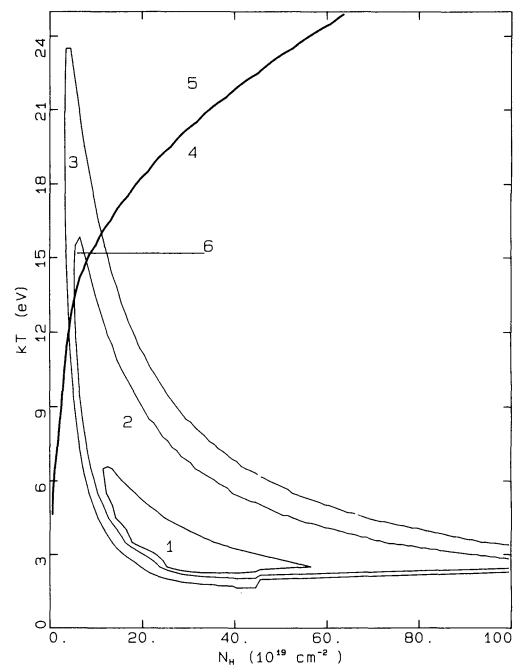
FIG. 4.—Determination of the parameters of the soft X-ray blackbody. The various regions are labeled as explained below. From the X-ray (LE filter ratio) data we can construct three regions: (1): hole inside region 2—allowed only by 4000LX over A1/P ratio, but excluded by 3000LX over A1/P ratio; (2) “good” region—allowed by both the 3000LX over A1/P and the 4000LX over A1/P ratios; (3) strip around region 2—allowed by the 3000LX over A1/P ratio, but excluded by the 4000LX over A1/P ratio. From the UV measurements we can divide the plane in two regions: (4) the one below the thick curve is excluded since the flux predicted by the soft X-ray blackbody at 1300 \text{ \AA} exceeds the measured value of 2.9 \times 10^{-14} \text{ ergs cm}^{-2} \text{ s}^{-1} \text{ \AA}^{-1} ; (5) the one above is allowed by UV measurements. The intersection of regions 2 and 5 is region 6, which is allowed by both X-ray and UV measurements.
