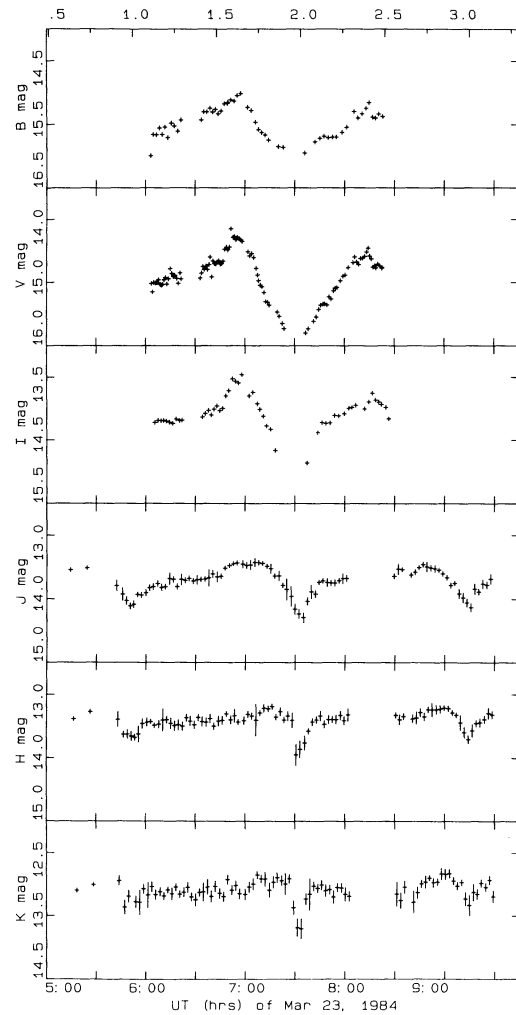
FIG. 8.—Light curves in the B , V , I , J , H , and K bands of 1984 March 23. Top frame axis is labeled in phase.
